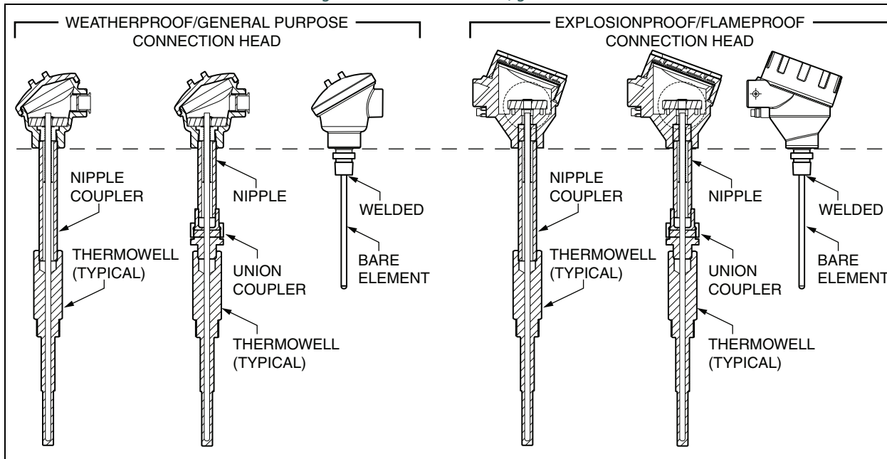
Figure 1. PR Series RTD Configurations
