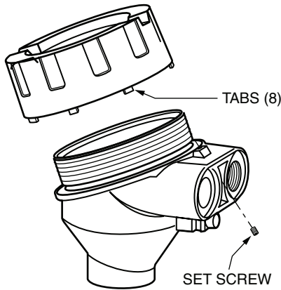
Figure 7. Cover Lock
