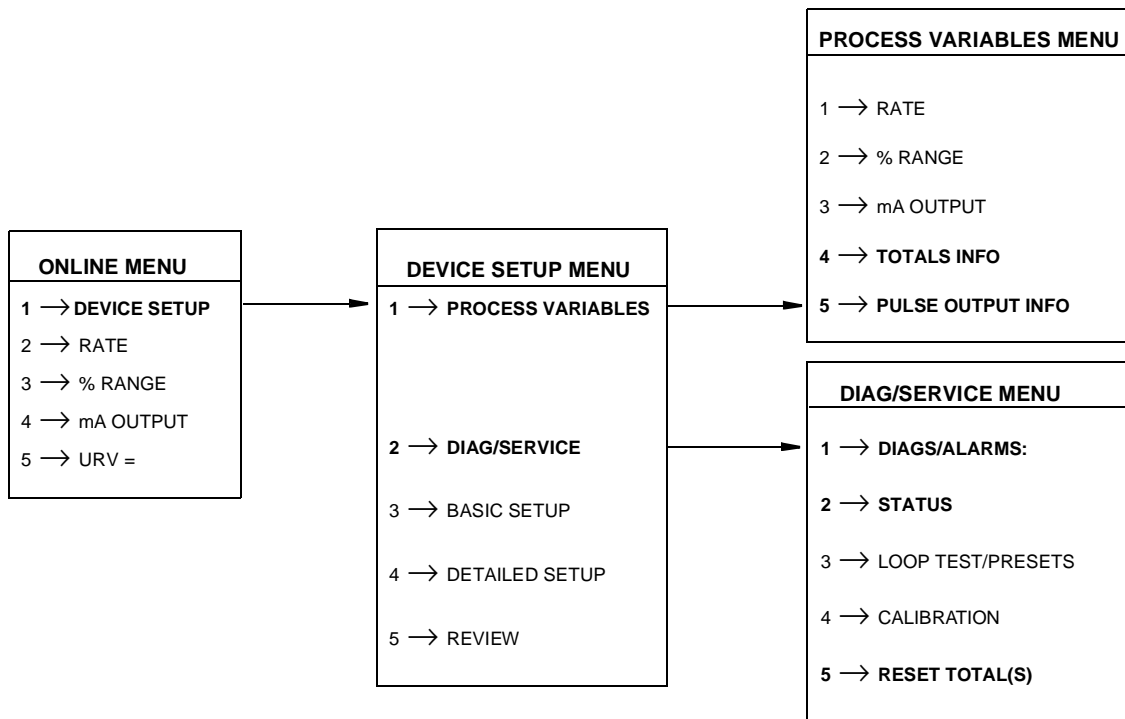
Figure 3. Menu Structure for Normal Operation
