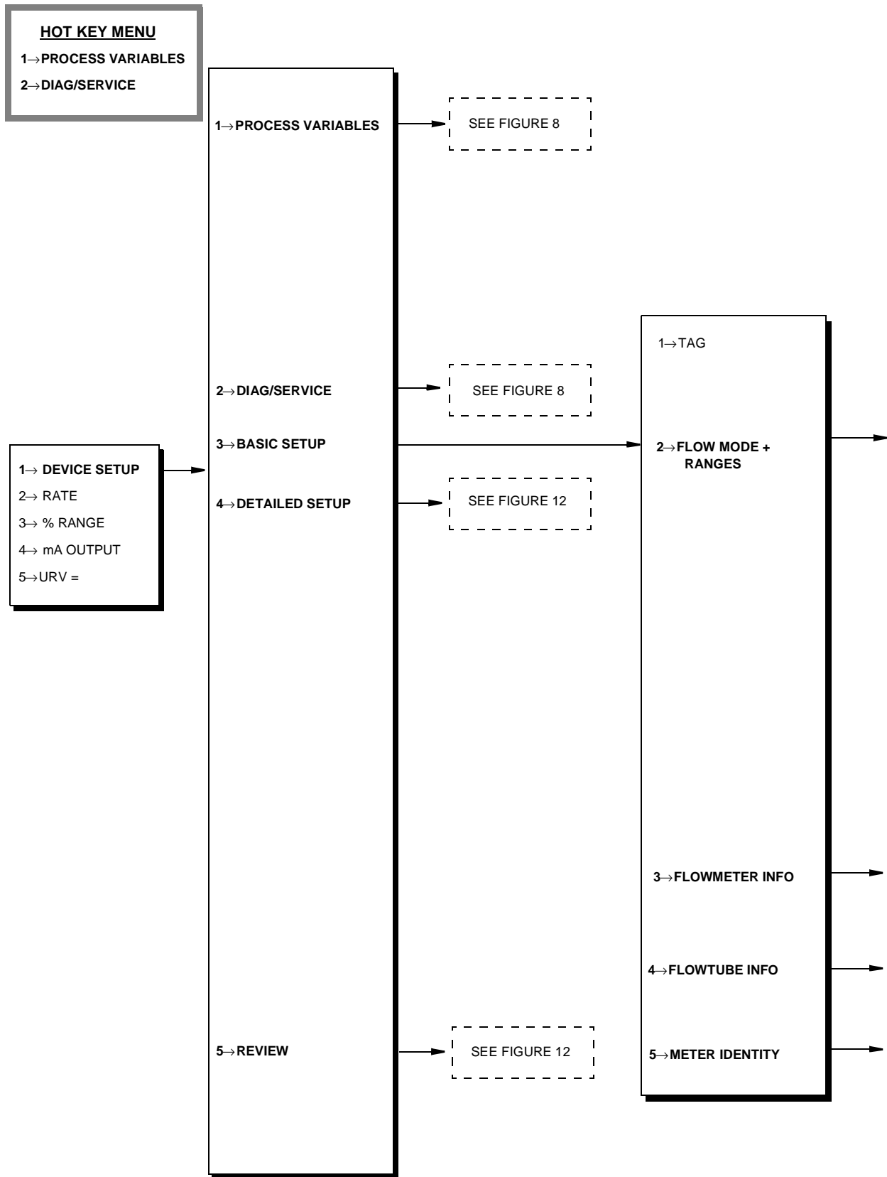
Figure 10. Menu Structure Diagram for Basic Setup (1 of 2)
