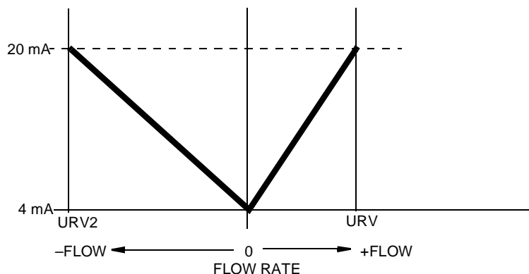
Figure 5. BiDirectional Dual Range Milliamp Output
