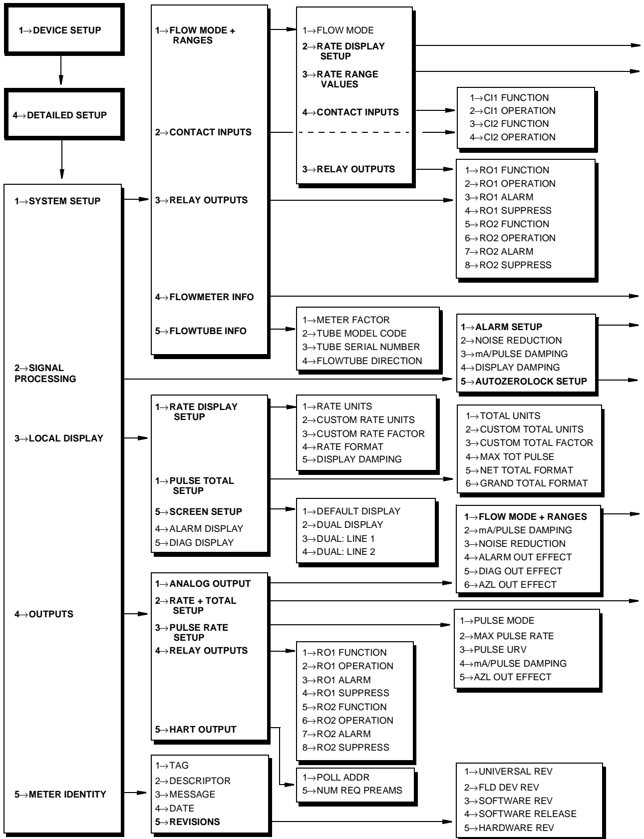
Figure 12. Menu Structure Diagram for Detailed Setup (1 of 2)
