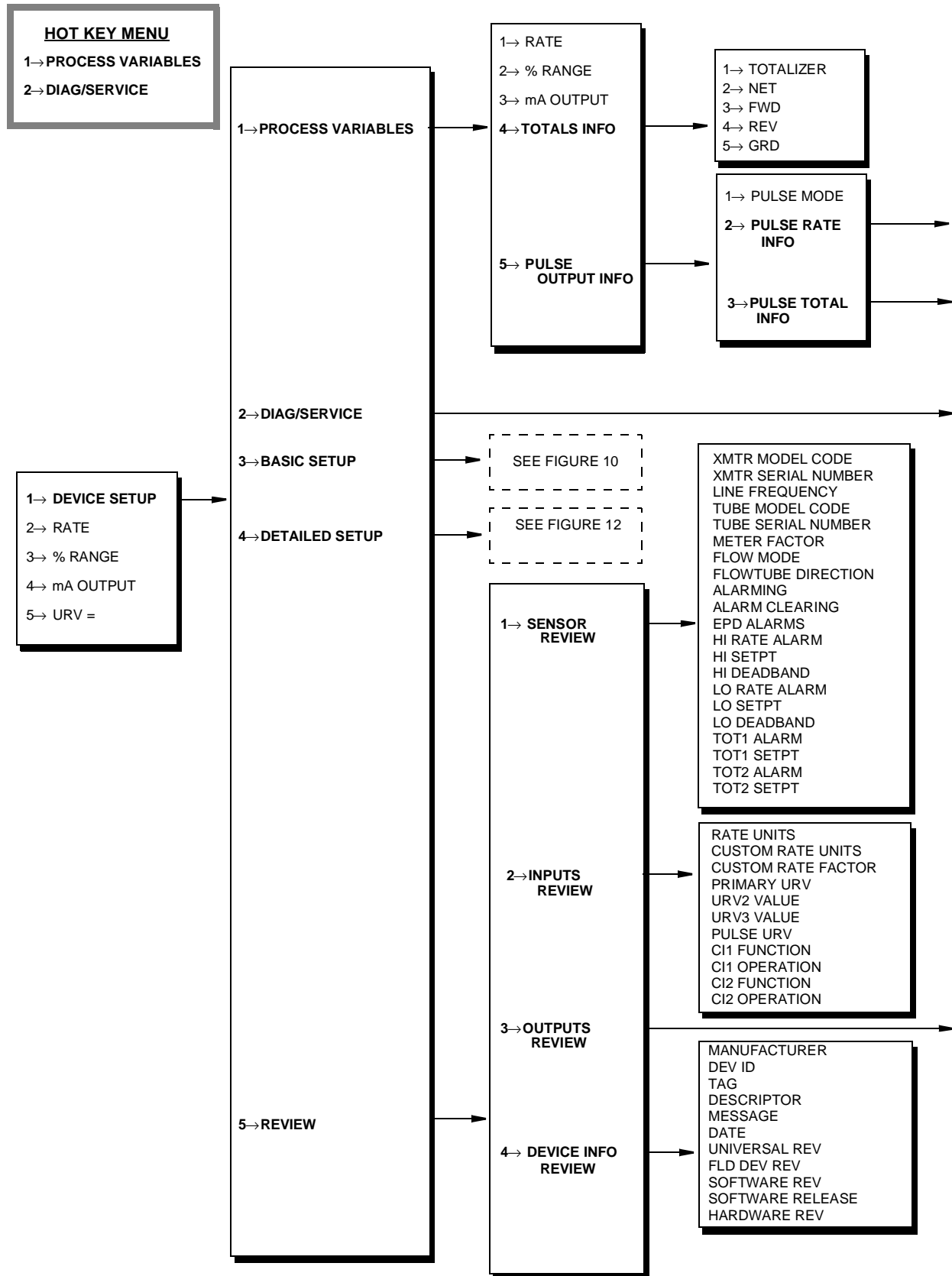
Figure 8. Menu Structure Diagram for Operation, Calibration, Presets, and Review (1 of 2)
