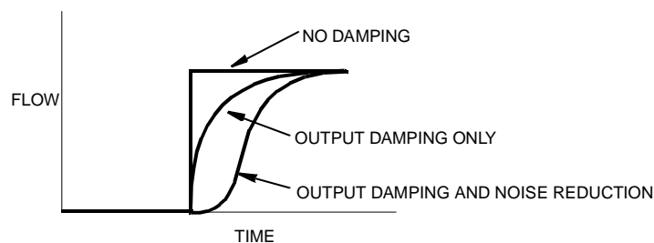
Figure 7. Noise Reduction
