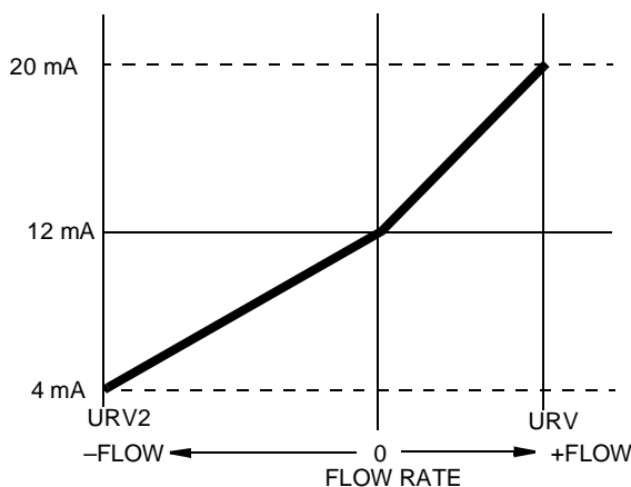
Figure 6. BiDirectional Split Range Milliamp Output
