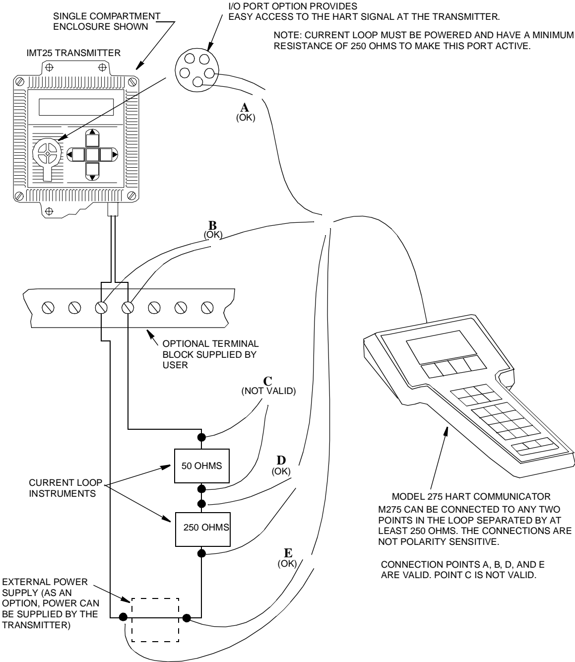
Figure 1. Model 275 Connection Diagram
