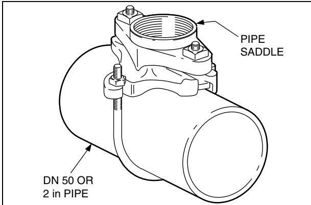
Figure 33. Leveling Pipe Saddle
