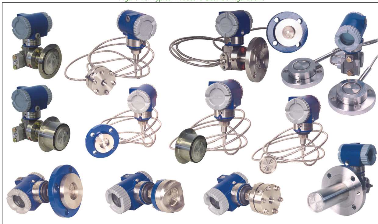
Figure 40. Typical Pressure Seal Configurations
