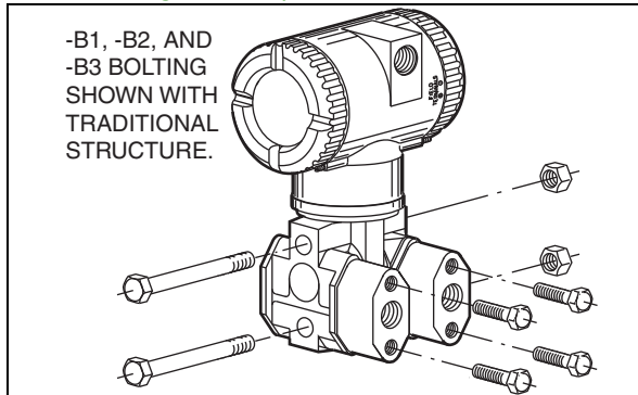
Figure 12. Options -B1, -B2, and B3
