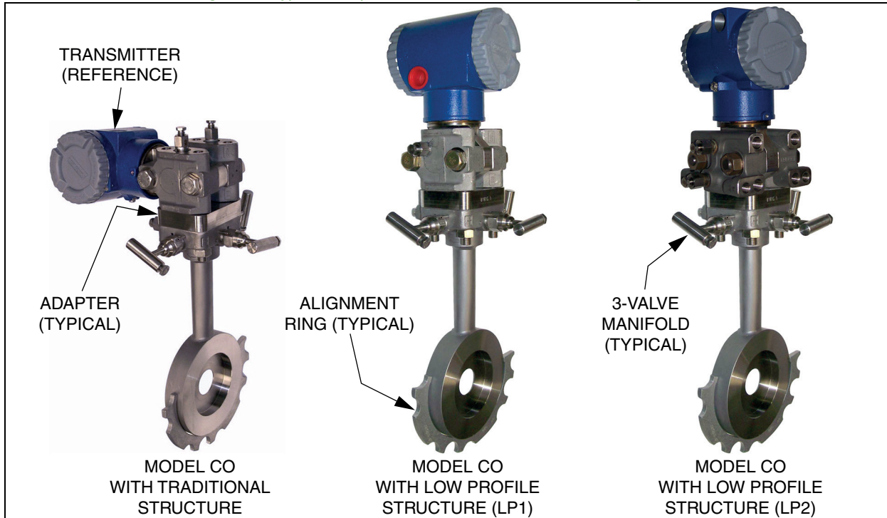
Figure 37. Typical Compact Orifice/Manifold/Transmitter Configurations
