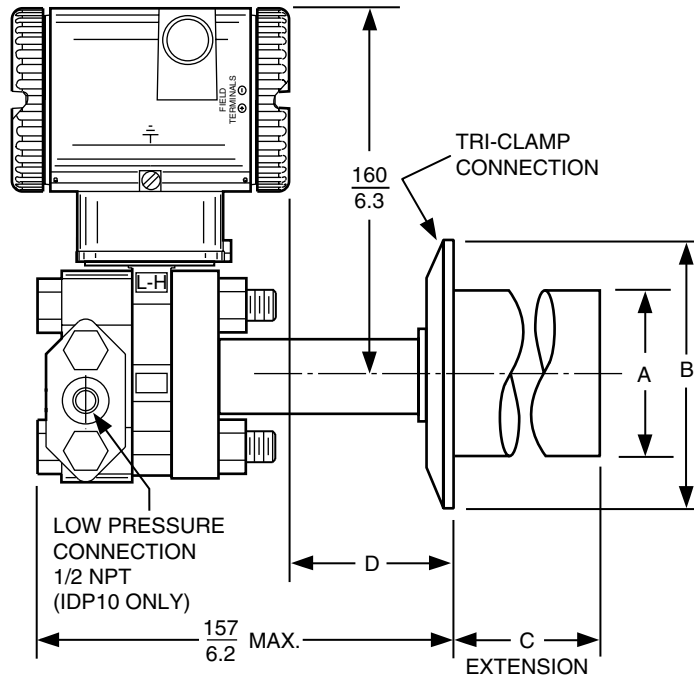
PRESSURE SEAL DIMENSIONS
