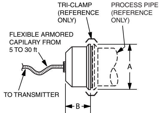
PRESSURE SEAL DIMENSIONS
