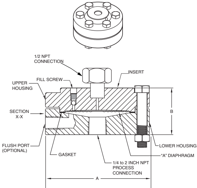
PSTAR AND PSTAD 2.4 AND 2.9 in DIAPHRAGM
