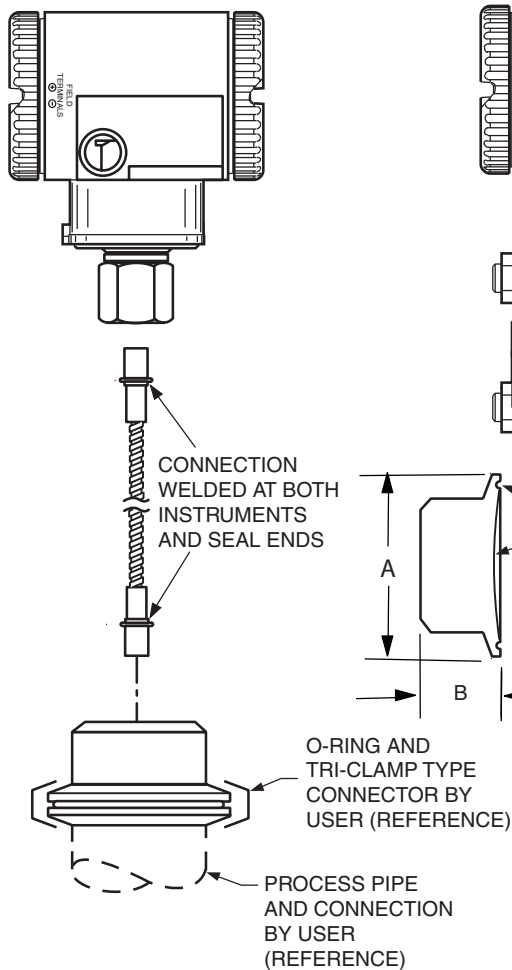
PSSCR SHOWN WITH IGP10 TRANSMITTER
