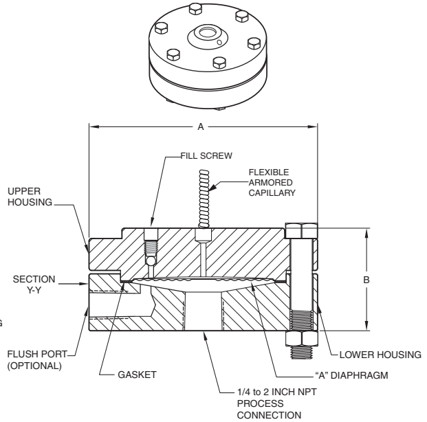
PSTAR ONLY 4.1 in DIAPHRAGM
