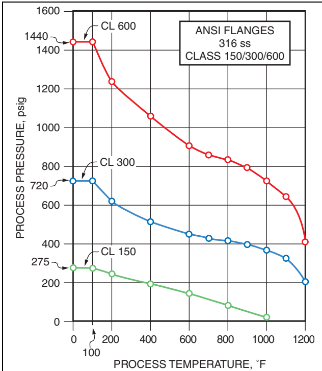
Figure 1. Pressure-Temperature Limits of Model TF
