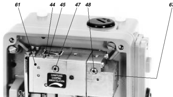
Double-acting Positioner SRI986
