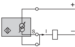
2-wire connection
