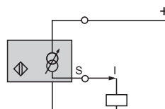
3-wire connection
