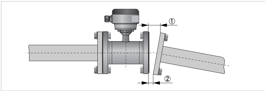
Figure 2-16: Flange deviation
