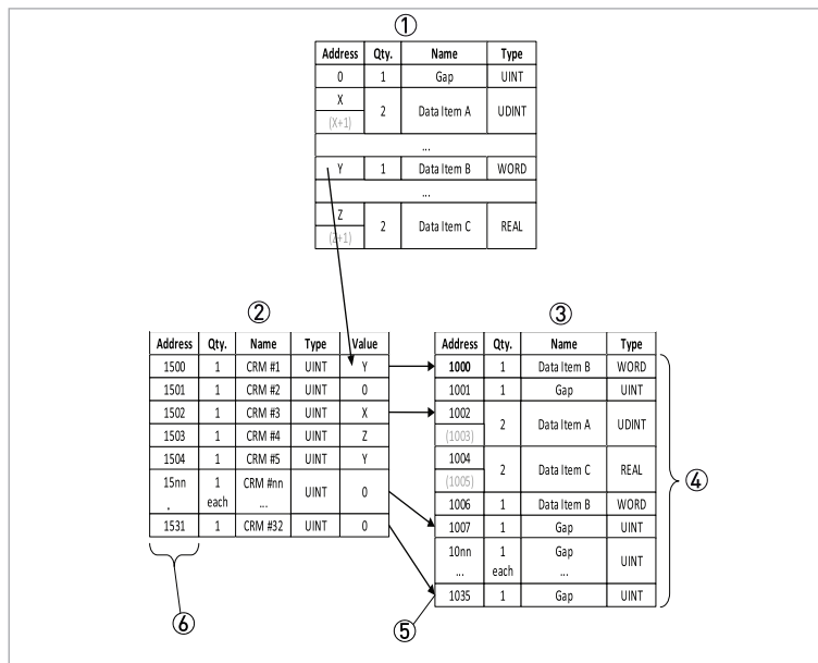
Figure 6-6: Modbus Custom Register Assignment
