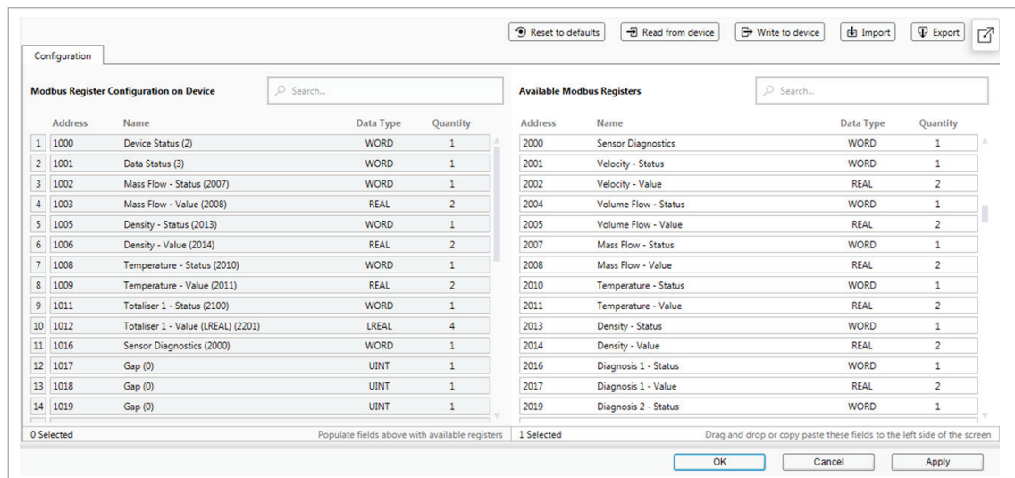
Figure 6-7: DTM Plugin for Modbus Custom Register Assignment
