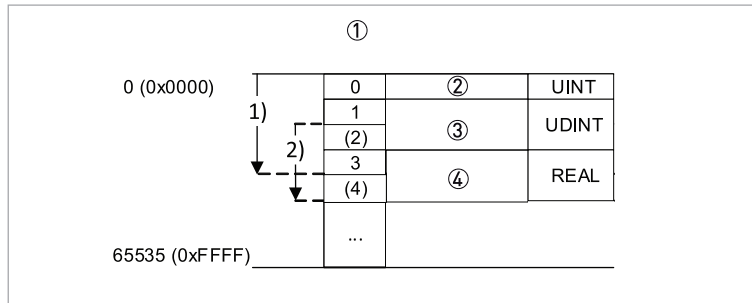
Figure 6-4: Modbus data mapping - Example (invalid access)
