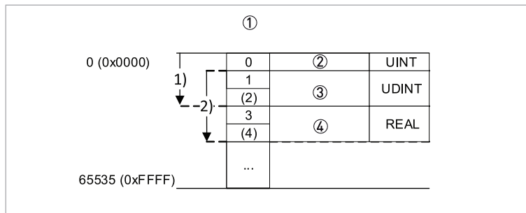
Figure 6-3: Modbus data mapping - Example (valid access)
